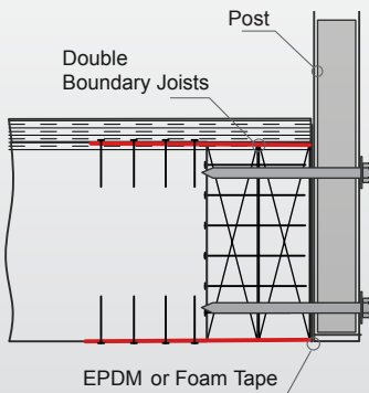
FACE FIX TO STEEL
