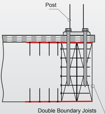
TOP FIX TO TIMBER
