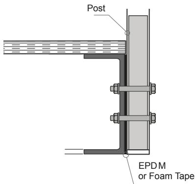
TOP FIX TO TIMBER
