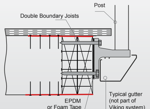
FACE FIX TO TIMBER WITH GUTTER BRACKET
