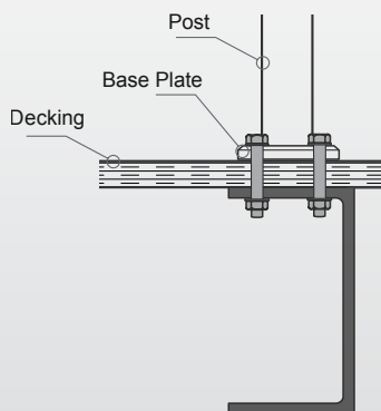
TOP FIX TO TIMBER DECK AND STEEL
